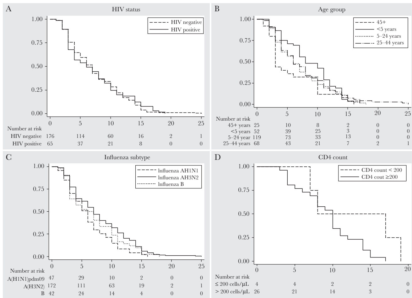
Figure 2. Kaplan-Meier plots showing the probability of reverse transcription polymerase chain reaction-positive influenza virus result by day after shedding onset by (A) human immunodeficiency virus (HIV) status, (B) age group, (C) influenza subtype, and (D) CD4 count.
